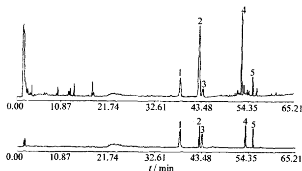
1-三七皂苷 R 1 2-人参皂苷 R g1 3-人参皂苷 R e 4-人参皂苷 R b1 5-人参皂苷 R d 1-notoginsenoside R 1 2-ginsenoside R g1 3-ginsenoside R e 4-ginsenoside R b1 5-ginsenoside R d
